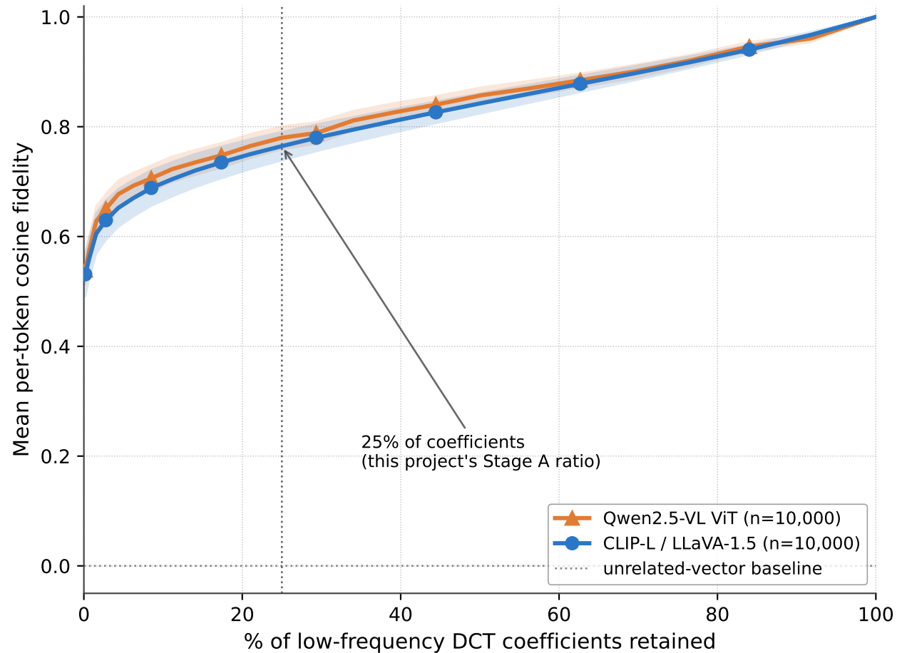
(b) Vision tokens are low-frequency redundant in two unrelated encoders
